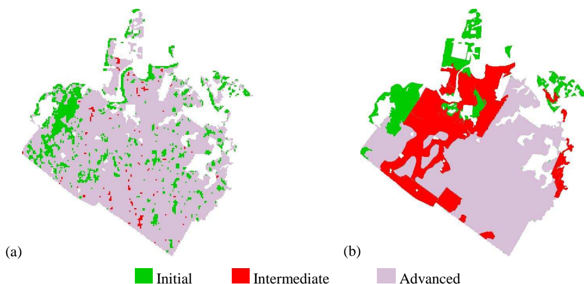
Figure 4. (a) Vegetation classification map derived from the analysis, and (b) reference map used to assess the classification accuracy.
