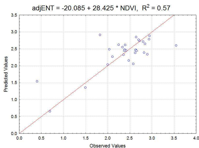
Figure 2. Resulting regression model (field ENT as a function of NDVI), and scatterplot of predicted versus observed values.
