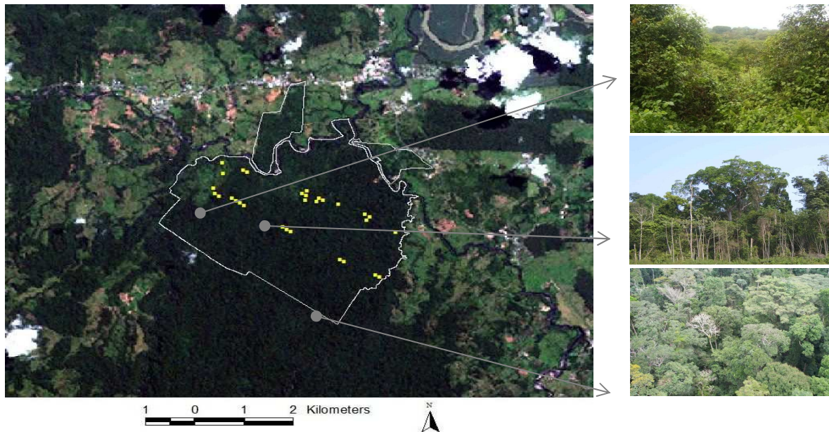
Figure 1. Landsat ETM+ image (R3-G2-B1 composite) of La Selva Biological Station in Costa Rica, outlined in white. The yellow dots are the locations of the 30 sample plots used in this work.
